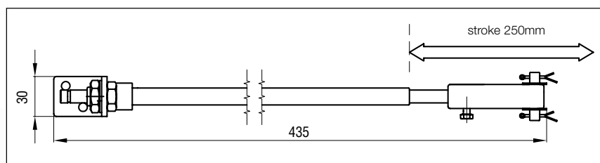
Fork dimensions
