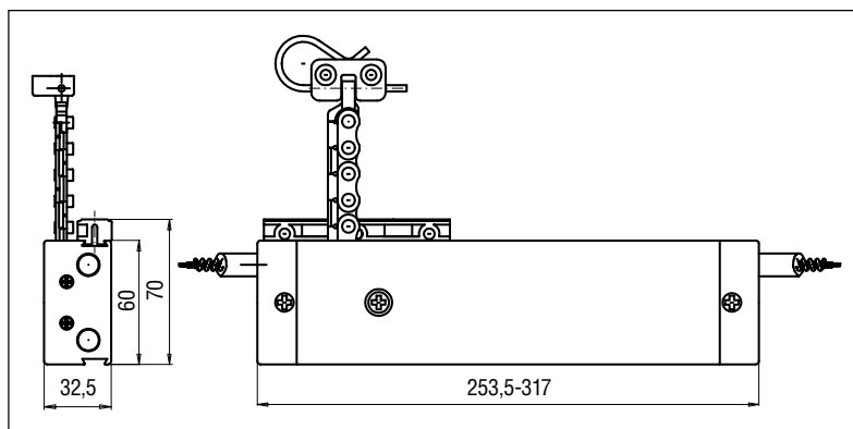
Mechanism dimensions
